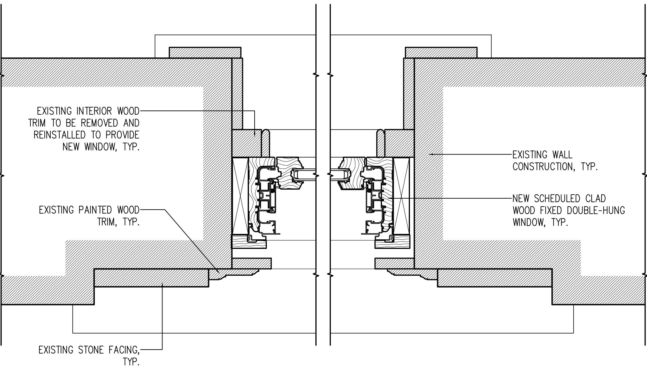
MONUMENTAL DOUBLE HUNG PLAN SECTION – STONE FRAMED OPENINGS
