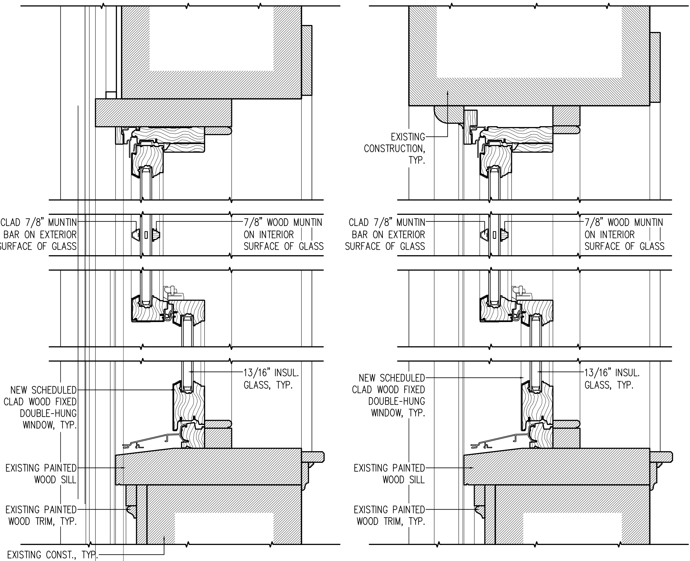
MONUMENTAL DOUBLE HUNG PLAN SECTION STONE FRAMED OPENINGS
