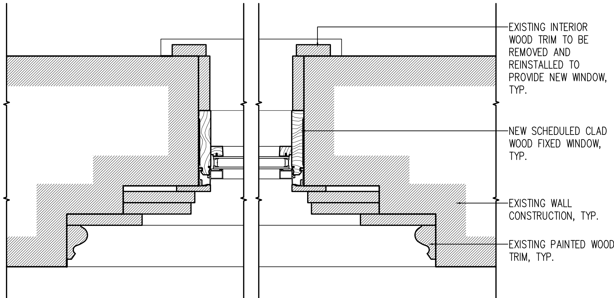
FIXED WINDOW PLAN SECTION
