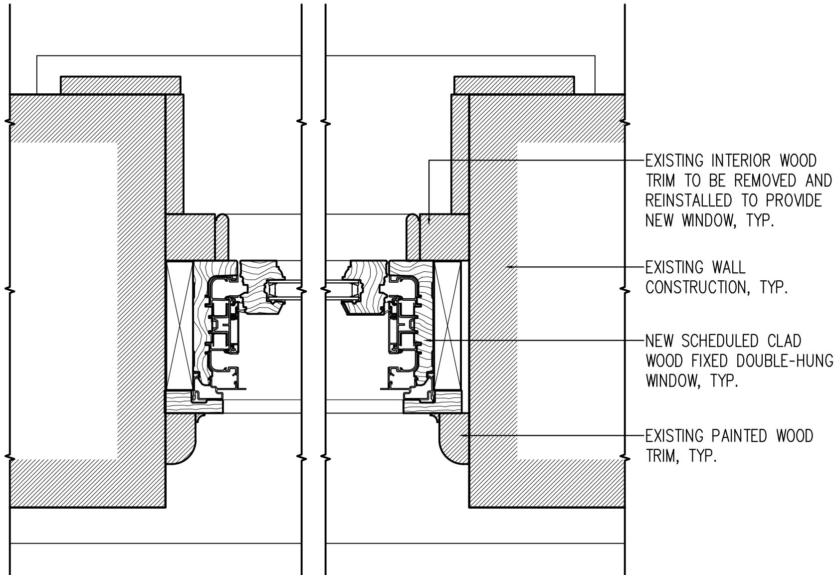
MONUMENTAL DOUBLE HUNG PLAN SECTION – BRICK MASONRY OPENINGS
