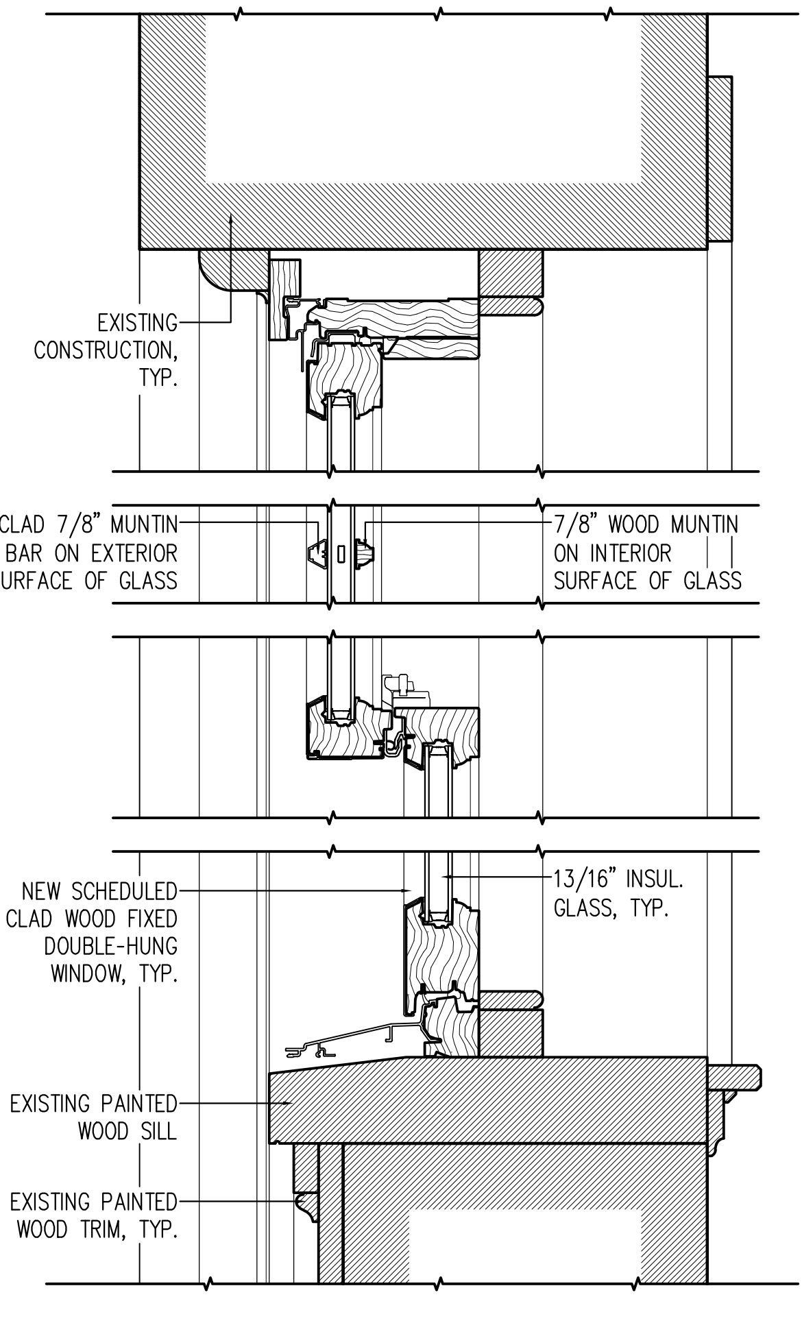
MONUMENTAL DOUBLE HUNG PLAN SECTION BRICK MASONRY OPENINGS
