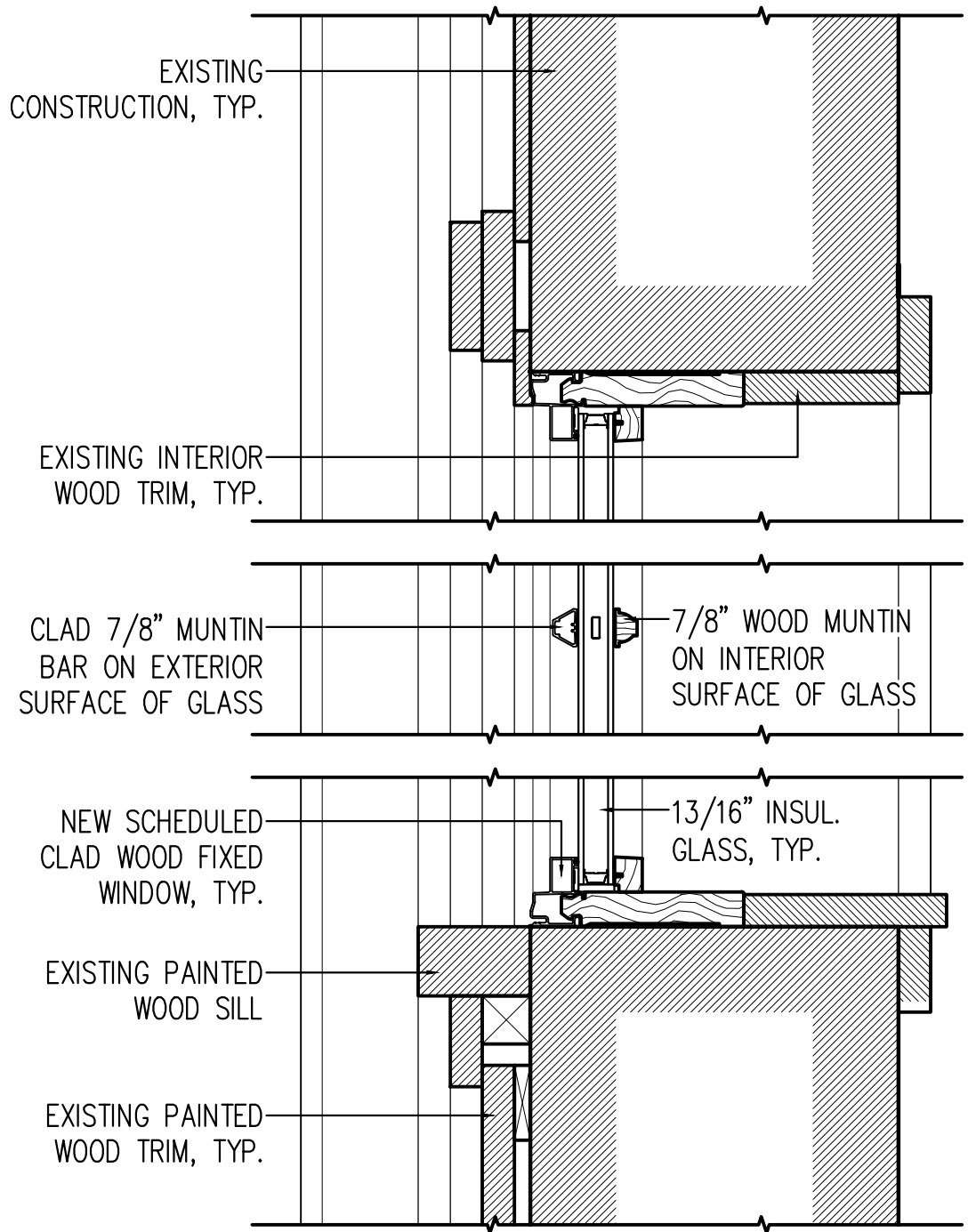
FIXED WINDOW SECTION
