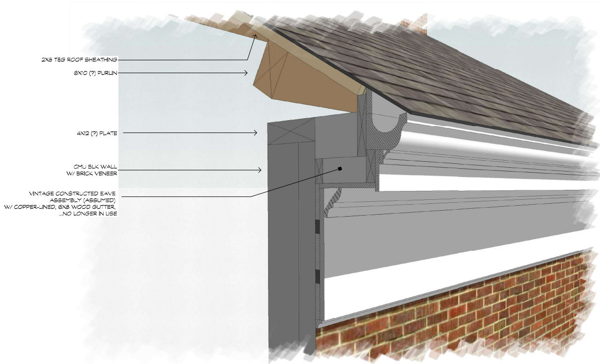
EXISTING, TYP.
